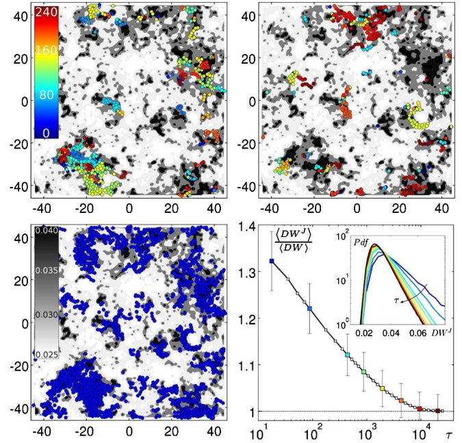
FIG. 2 (color online). Top: Cage jumps occurring between t and t + \tau_S for two different isoconfigurational trajectories, on top of a DW factor map computed at time t . Bottom left: Cage jumps occurring in 6 isoconfigurational trajectories between t and t + \tau_S tile the high DW regions. Color bar indicates the DW values in levels of gray. Bottom right: Average \langle (DW)^J \rangle over the particles having jumped between t and t + \tau , divided by the average \langle DW \rangle over all particles, as a function of the lag time \tau . Inset: PDF of (DW)^J for the particles jumping in [t; t + \tau] for several values of \tau . The black curve is the PDF for all particles.
