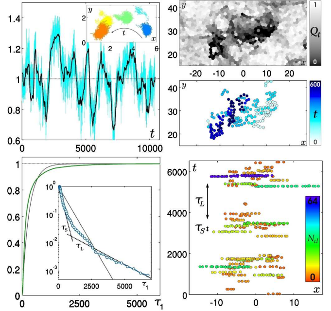
FIG. 1 (color online). Cage jump spatiotemporal organization. Top left: Comparison between the relative averaged relaxation Q_t(a^*, \tau^*) / \langle Q_t \rangle_t [gray (cyan)] and the relative percentage P_t(\tau^*) / \langle P_t \rangle_t of particles that have not jumped between t_0 and t_0 + \tau^* (black). Inset: Trajectory of a single particle over 14\tau_\alpha . Color changes when the particle jumps. Top right: (inner top) Map of Q_t(\tau^*) ; (inner bottom) particles having jumped during the same lag \tau^* ; jumping time is color-coded. Bottom left: Cumulative probability distribution function of the lag between adjacent clusters \tau_1 (thick green curve), compared to the corresponding curve for a random distribution of clusters (black). Inset: PDF of \tau_1 (circles). The exponential distribution with same mean is shown for comparison (solid line), as well as exponentials of typical time scale \tau_S and \tau_L (dotted lines). Bottom right: Spatiotemporal view of the cage jumps in a specific region of space, projected on the x axis. The cluster size is color-coded. Note the aggregation of clusters in avalanches. The typical time scales of the dynamics are shown.
